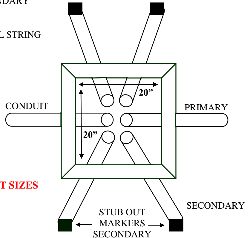
TOP VIEW OF VAULT
